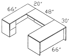
RU-EU6630 L/R 'U' W/66\" Return-Left or Right
