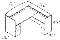
RU-RUTRT L/R Reception Unit W/Transaction Return Top
