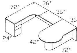
RU-EUPT3624CC L/R 'U' W/P-Top W/Corner Credenza-Left or Right
