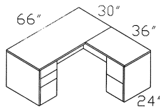
RU-EL663036 L/R 'L' W/36" Return-Left or Right
