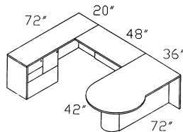
RU-EUPTCOM L/R 'U' W/P-Top W/Combo Lateral File -Left or Right
